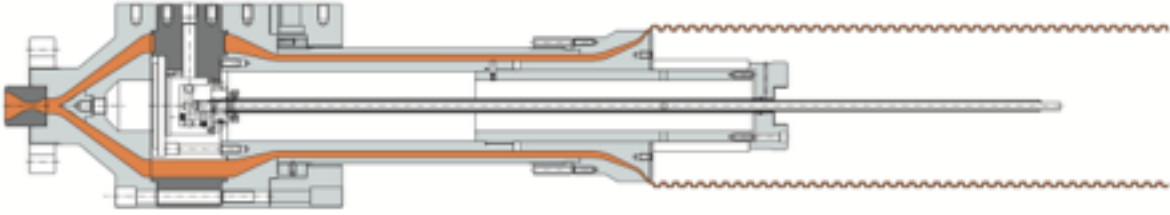
Single Wall Pipe die.
