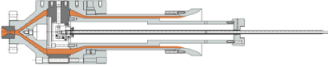
Corma's patented die prepared for exchangeable tooling.
