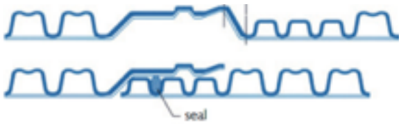
Bell and spigot double skin in-line coupling.
