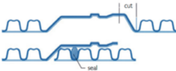
Standard double skin in-line coupling.
